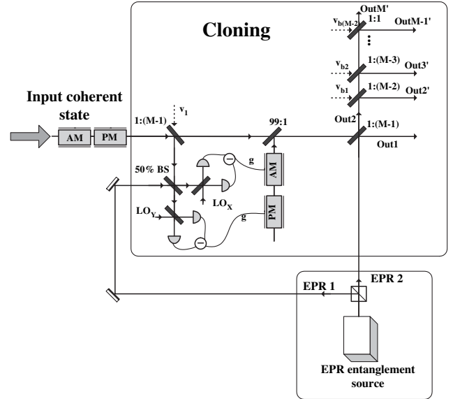
FIG. 3. Schematic of the quantum state transfer with partially disembodied transport viewed as 1 \rightarrow M optimal Gaussian cloning machine.
